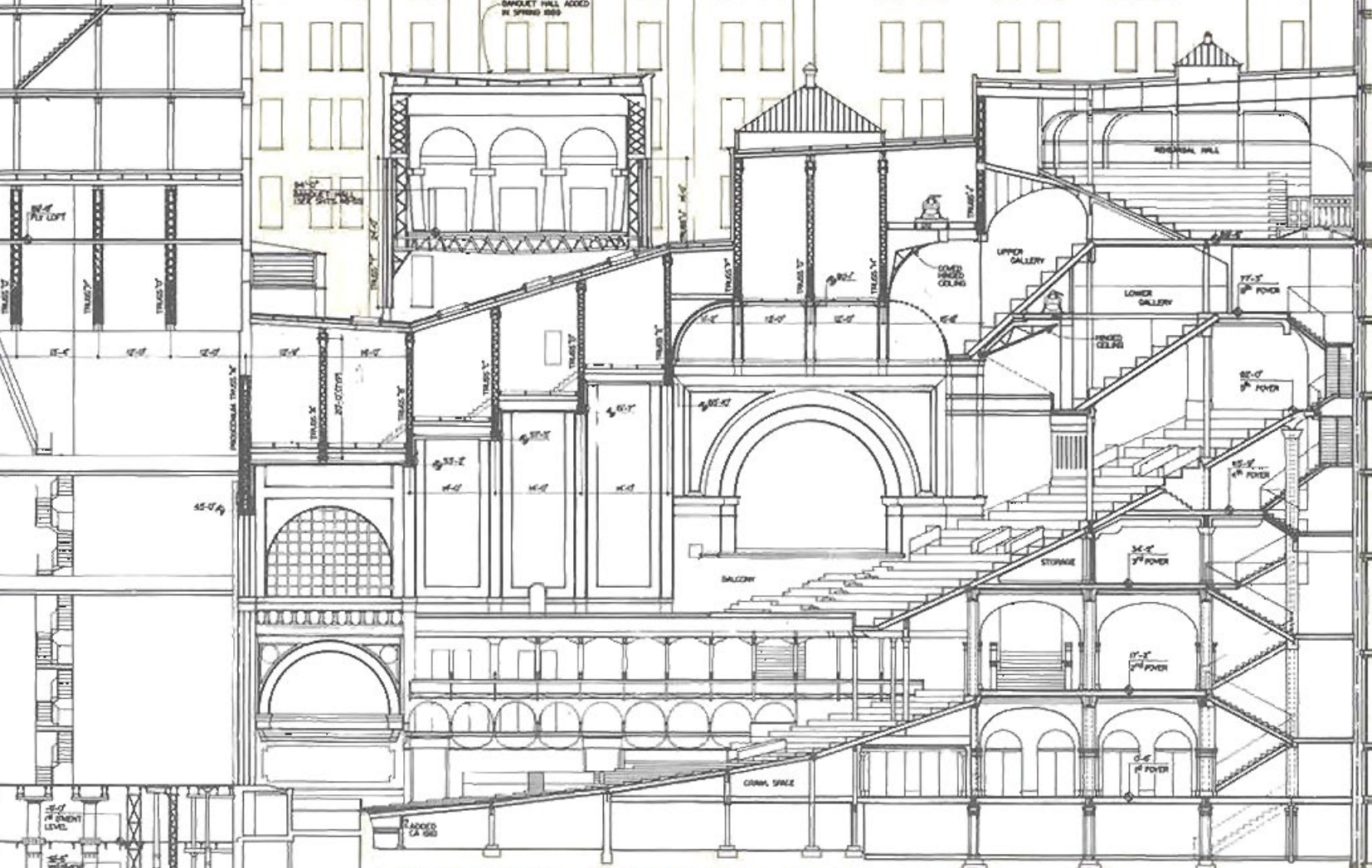
LONGITUDINAL SECTION XX LOOKING SOUTH AS COMPLETED IN 1890
